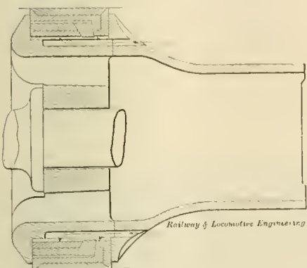
FIG. 14. "AMERICAN" ONE RING COMPLETE.
